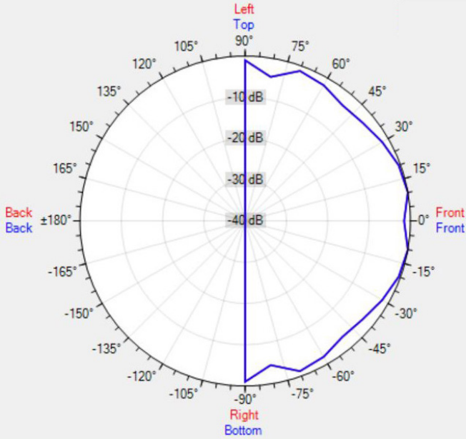
Data Shown: CM20T (Apart Audio) Display Parameters: Frequency: 1000Hz (1/24th Octave)
