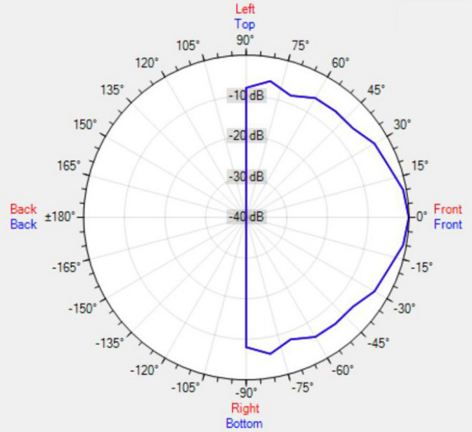
Data Shown: CM20T (Apart Audio) Display Parameters: Frequency: 2000Hz (1/24th Octave)
