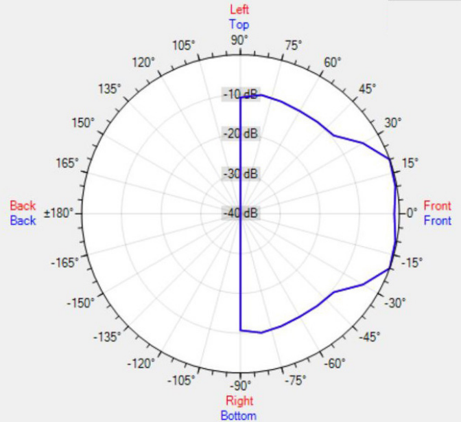
Data Shown: CM20T (Apart Audio) Display Parameters: Frequency: 8000Hz (1/24th Octave)
