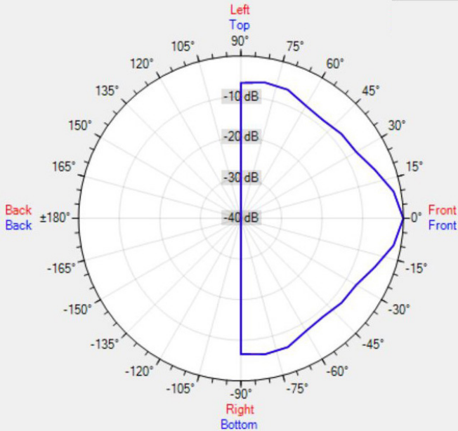
Data Shown: CM20T (Apart Audio) Display Parameters: Frequency: 4000Hz (1/24th Octave)
