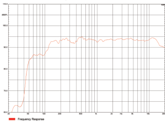
⊙ Artist T6 Frequency Response Curve
